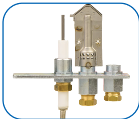
Group C Pilot Burners
