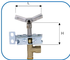
A Group Y Type Pilot Burners
