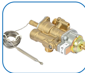
Thermostatic With Safety Gas Tap With Ignition Flame
